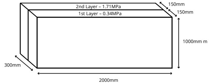
Figure 1: Full Width Deformable Barrier external dimensions
